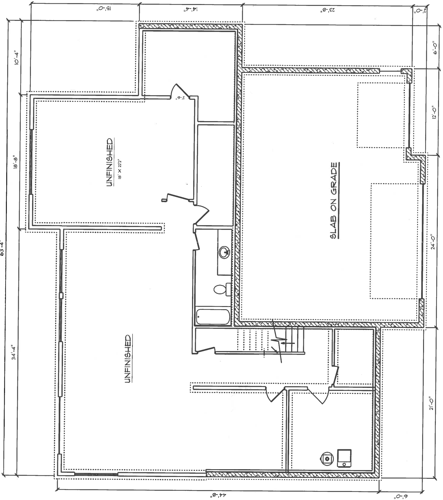
UNFIN BSMT. / FOUNDATION PLAN
